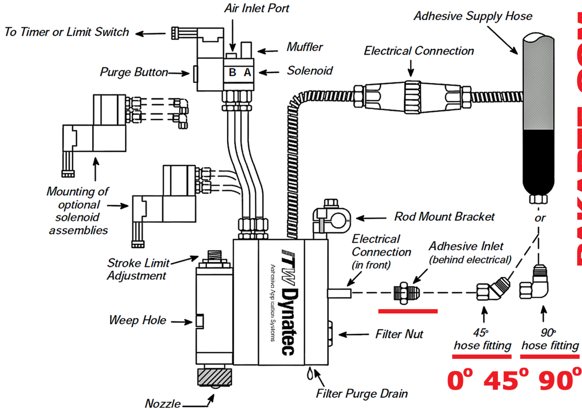
Installation Diagram
