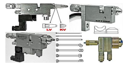
AS-AUTOMATIC VALVES-GUNS
