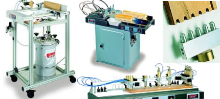
PZ-SEMI-AUTOMAT DEVICES
