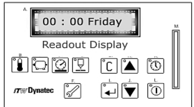
DynaControl® Keypad
