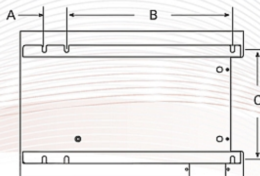
Mounting Hole Dimensions
